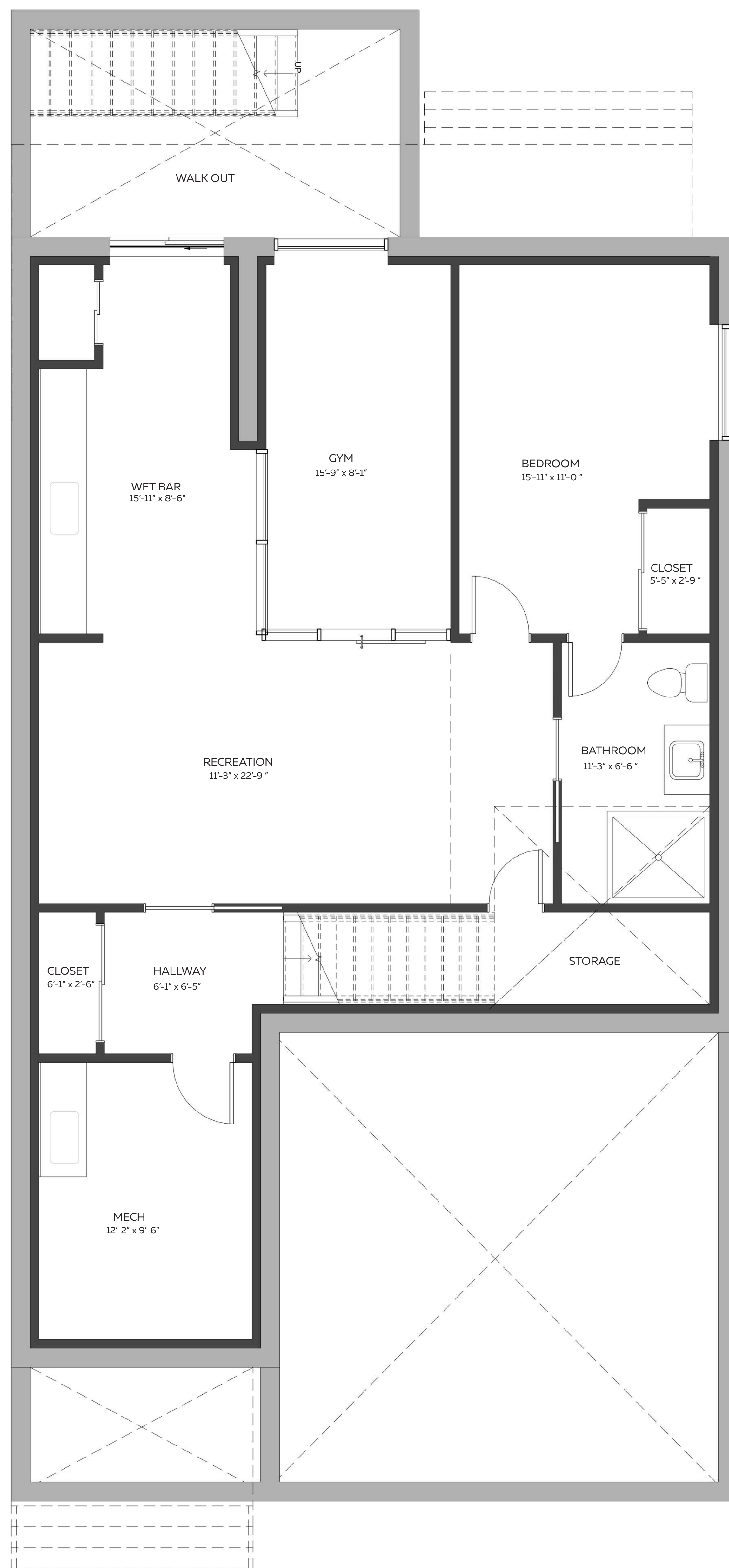
Basement
