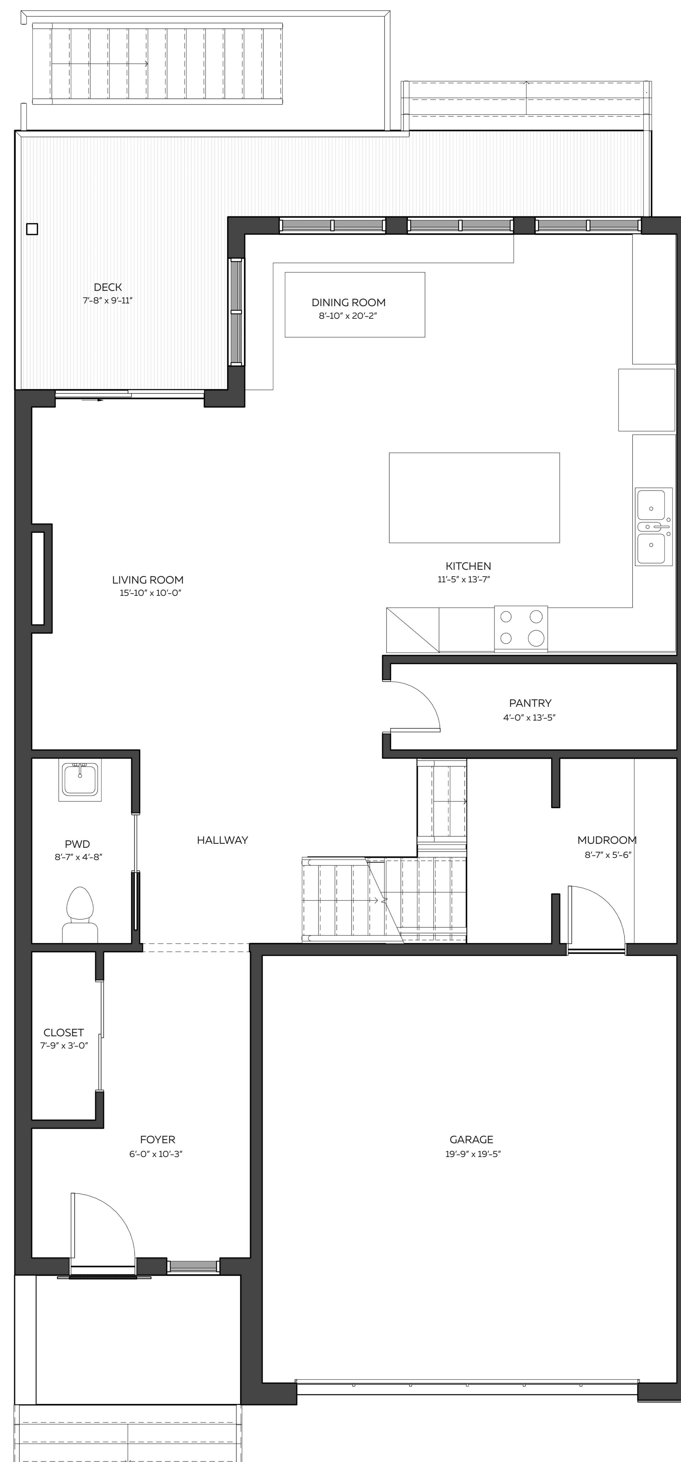
Main Floor
