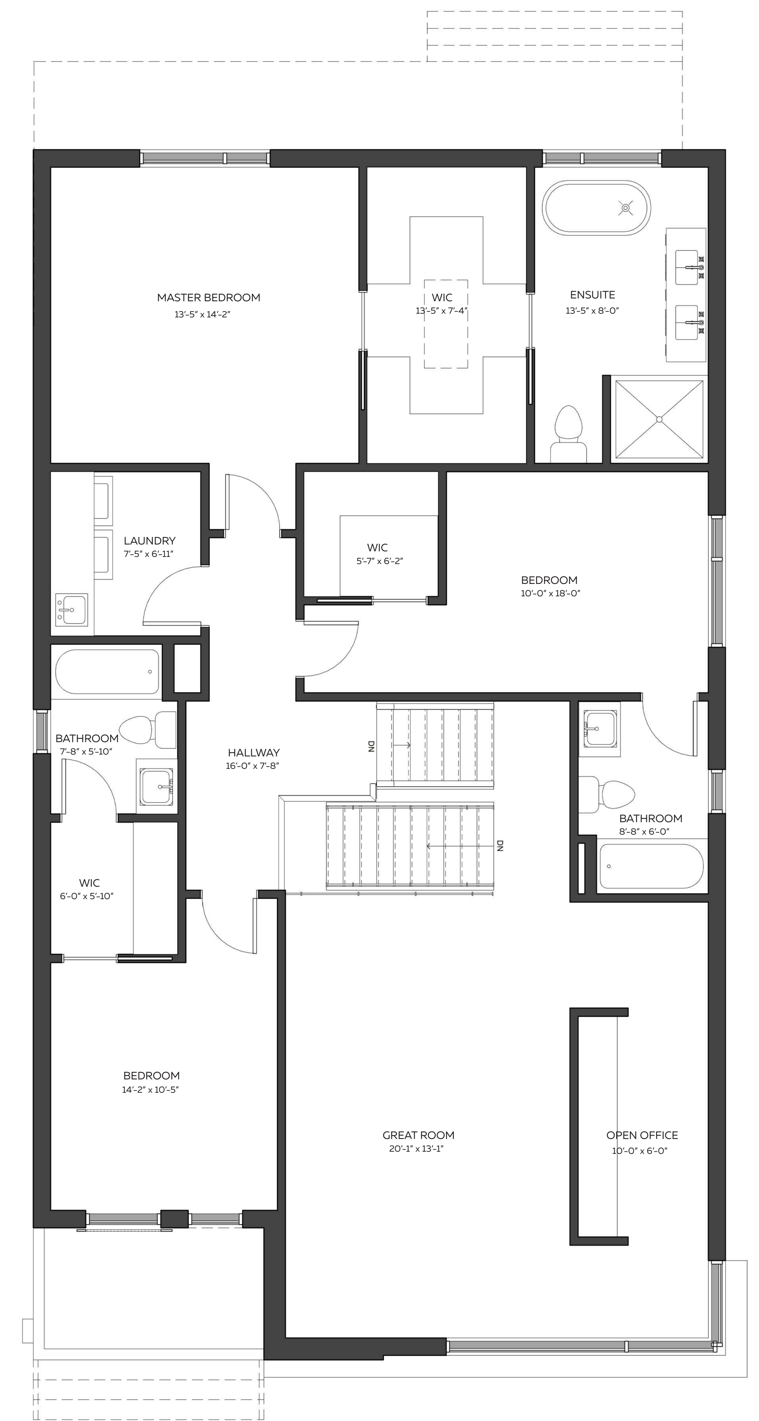
Second Floor
